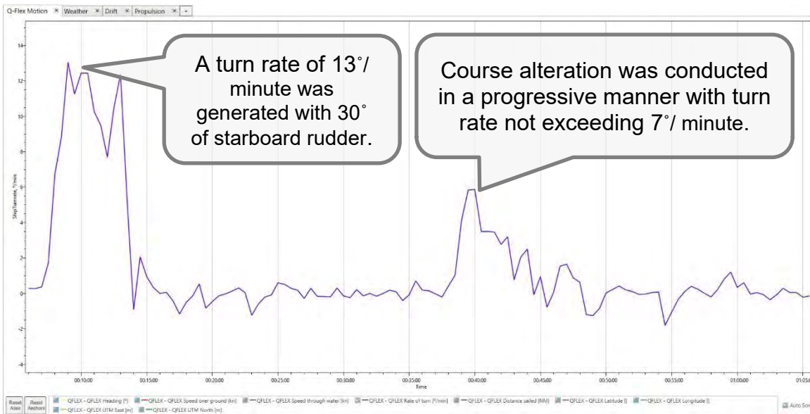
Figure 46: Rate of turn – outbound LNGC, wind SE 40 (R1-4)
