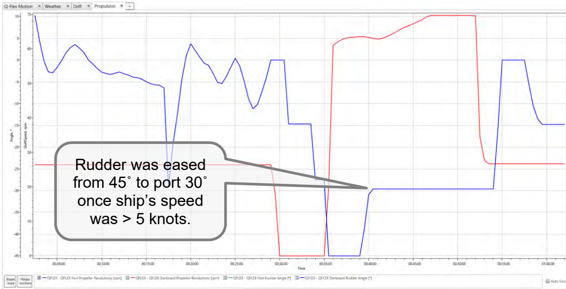
Figure 74: Rudder and RPM – turning stern through 50 knot winds (R1-10)
