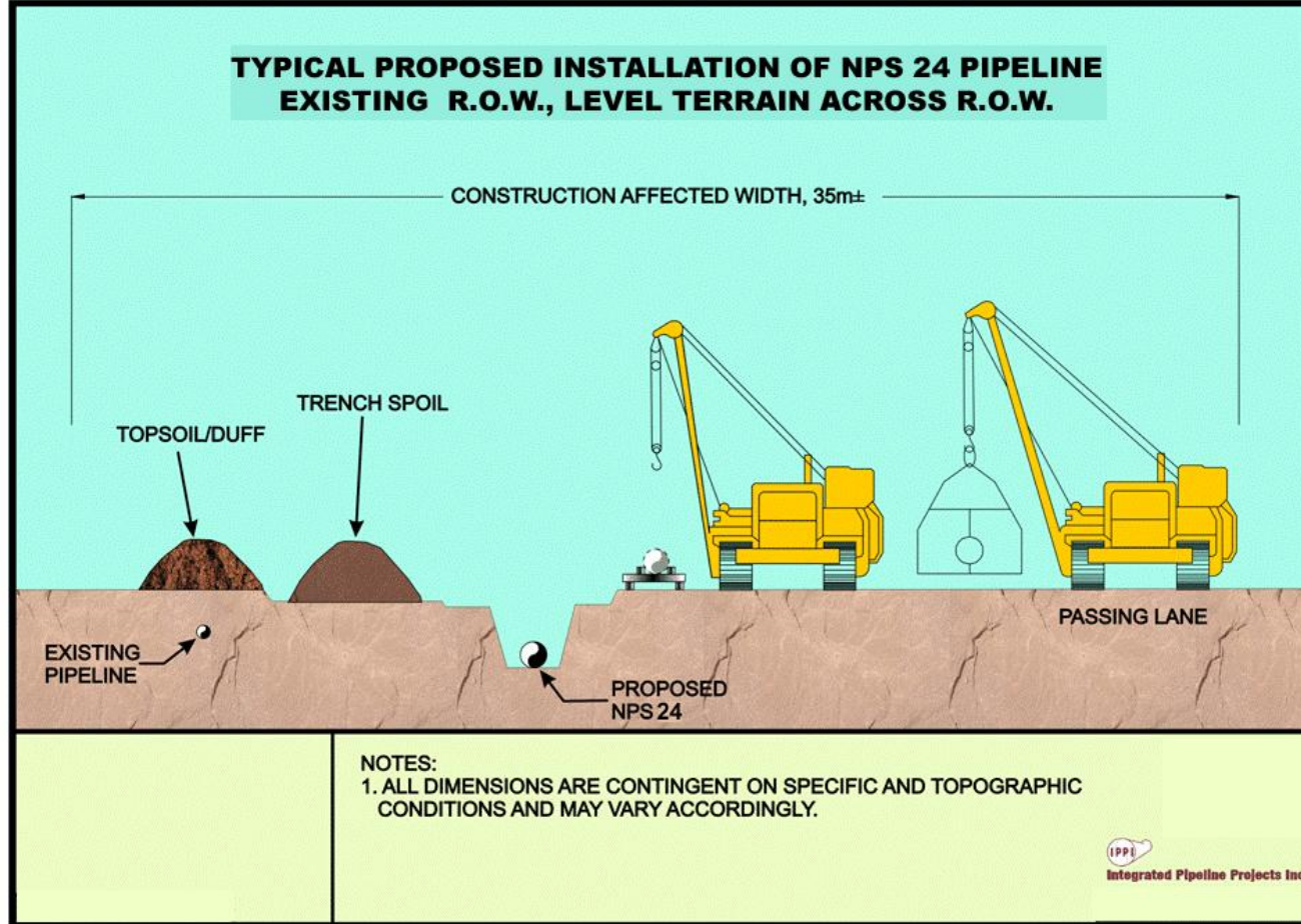
Figure 2. Typical pipeline installation method
